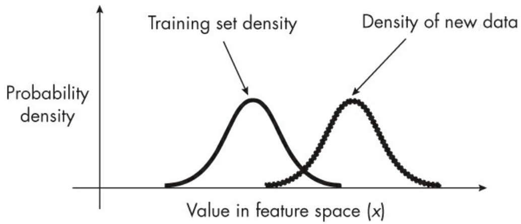
Figure 23-1: Training dat
